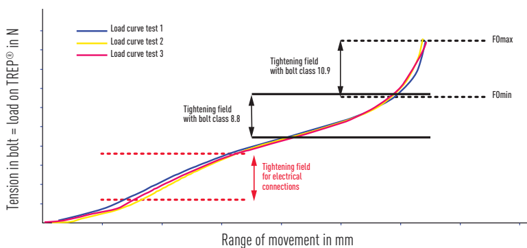
Load curves of TREP® 3L and tightening fields
